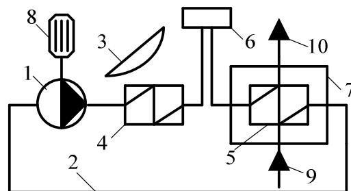
Figure 2. The new process scheme of electric generator air cooling and water heating: 1 – pump; 2 – water line; 3 – solar concentrator; 4 – absorption machine; 5 – water-air heat exchanger; 6 – heat water consumption; 7 – electric generator; 8 – electric drive; 9 – atmospheric air input; 10 – atmospheric air output
