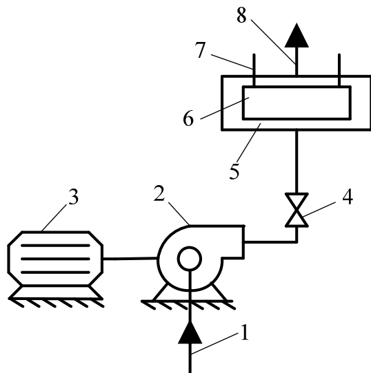
Figure 1. The process scheme of electric generator air cooling: 1 – atmospheric air input; 2 – centrifugal fan; 3 – electric drive; 4 – shutoff valve; 5 – electric generator; 6 – water-air heat exchanger; 7 – water; 8 – atmospheric air output
